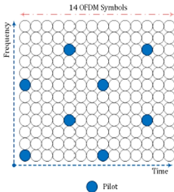
Figure 1-: An example of the time-frequency resource grid for LTE-A
