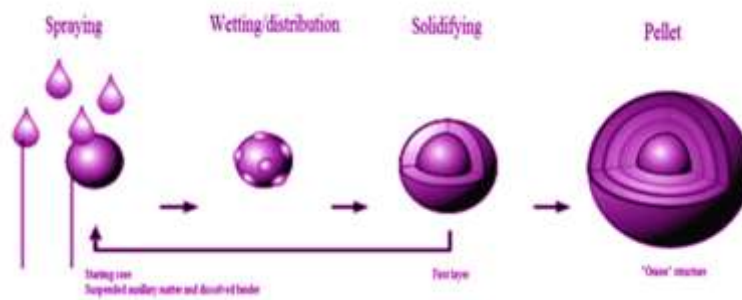
Figure 1: Principle of solution and suspension layering
