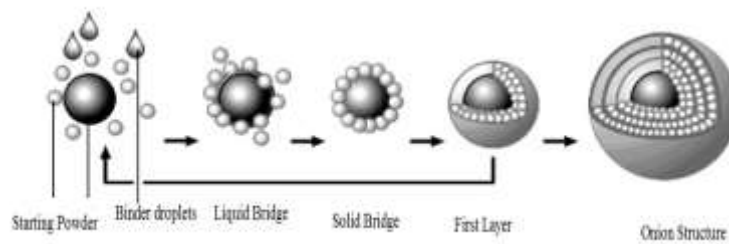
Figure 2: Principle of powder layering process.
